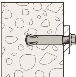
Undercut anchor FZA
