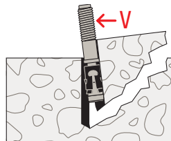
Pry-out failure
